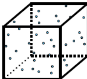
CLOUD
