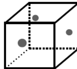
HAIL
