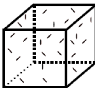
ICE
