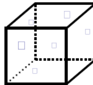
SNOW
