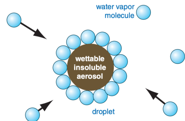
b) Heterogeneous nucleation
