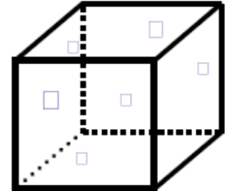
SNOW
