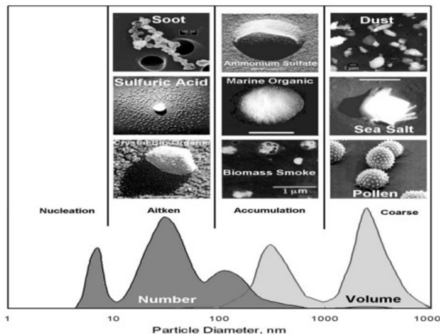
Figure 1 Typical shape of the aerosol number and volume size distribution, showing the various size classes ('modes') as well as example pictures of some archetypical aerosol particles. 1 nanometer (nm) = 0.001 micrometer; upper right value should read 10000 nm = 10 micrometer.
