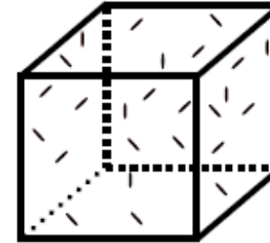
ICE
