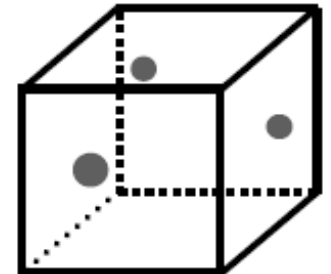
HAIL
