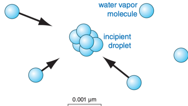
a) Homogeneous nucleation
