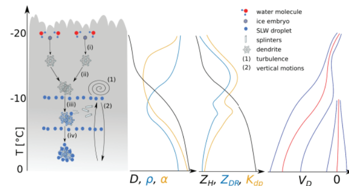
Figure 1.7 – Conceptual schematic of (i) vapour deposition, (ii) aggregation, (iii) early stage of riming, and (iv) later stage of riming (graupel). D is the hydrometeors' maximum dimension.
