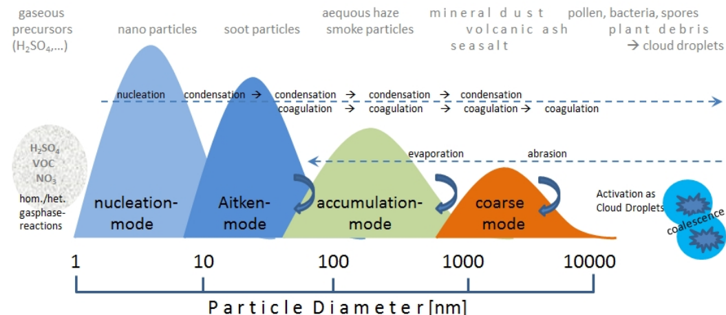
Figure 1 Typical shape of the aerosol number and volume size distribution, showing the various size classes ('modes') as well as example pictures of some archetypical aerosol particles. 1 nanometer (nm) = 0.001 micrometer; upper right value should read 10000 nm = 10 micrometer.
