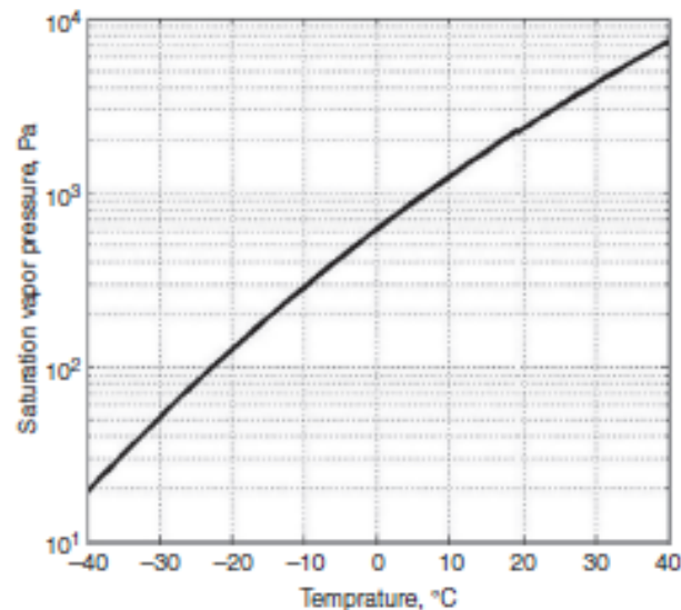
Figure 3.1.1 Dependence of saturation vapor pressure on temperature e_w(T_C) , calculated according to Flatau et al. (1992).
