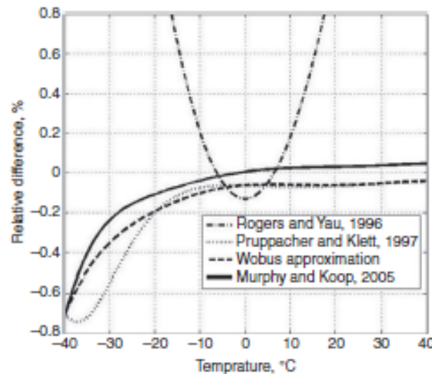
Figure 3.1.2 Relative difference (in percent) between the values of saturation vapor pressure e_w(T) with respect to values calculated by the formula suggested by Flatau et al. (1992) (see also http://cires.colorado.edu/~voemel/vn.html ).
