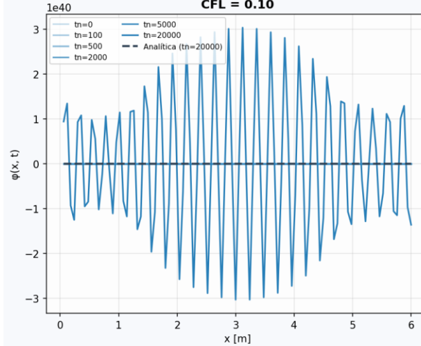
Esquema CTCS (Forward centrado) CFL = 0.10
