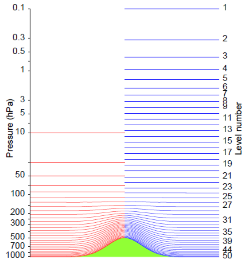
Figure 6. Vertical levels of the ECMWF model.
