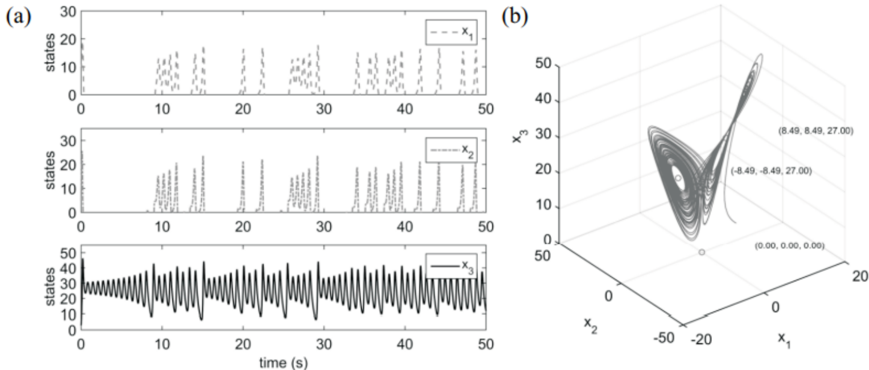
Figure 1. The chaotic behavior of the Lorenz system with initial point (10, 5, 3) . (a) x_1 , x_2 and x_3 are unstable vs. time. (b) The trajectory attract to none of fixed points. This system has three fixed points as listed in Table 1.
