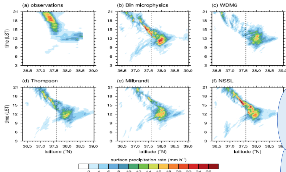
Latitude–time diagrams (Hovmöller diagram)
