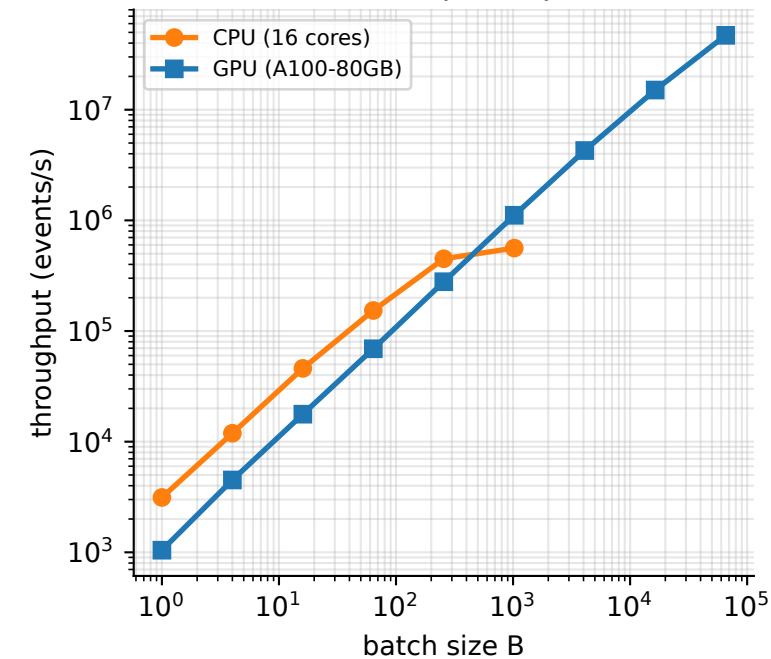
§4.3.1 GPU 84× speedup @ B=65K
