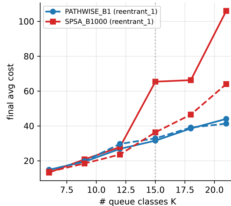
§5.3 Admission: PATHWISE scales, SPSA collapses at K \geq 15
