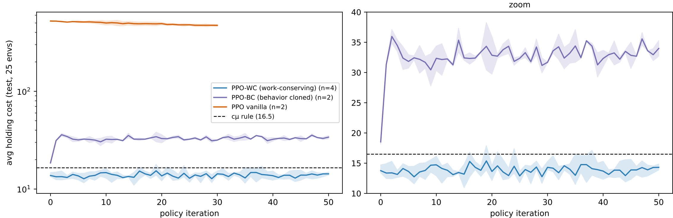
Fig 12 reproduction, multi-seed (reentrant_2 / 6 classes; SB3 PPO; episode_steps=15000 x 50 iters, reduced from paper 50000x100)
