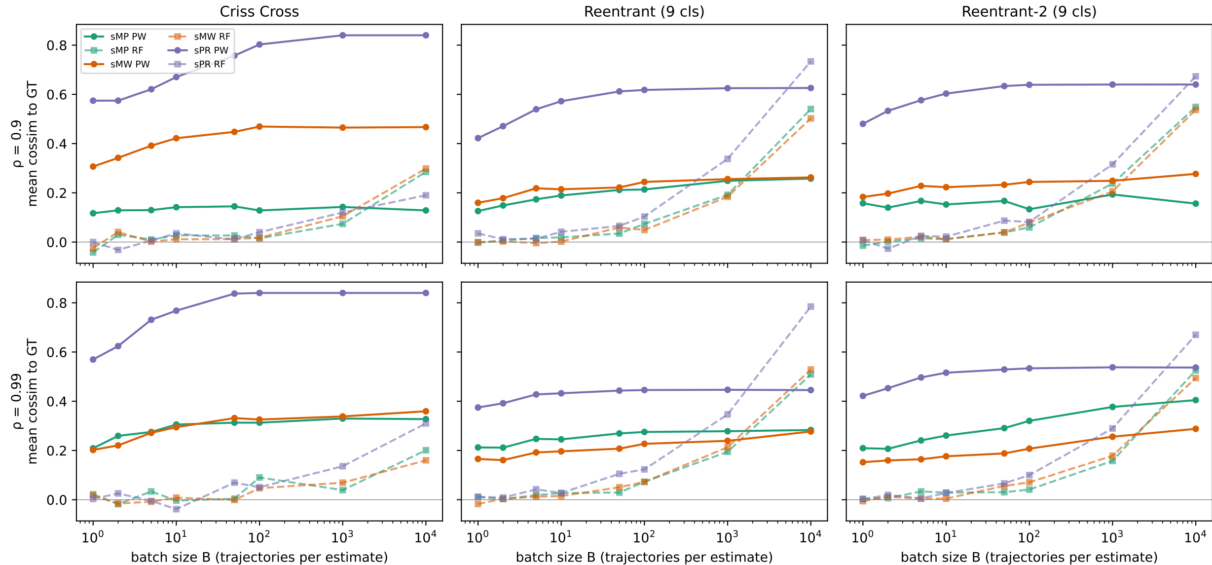
Cosine similarity vs batch size — PATHWISE (solid) vs REINFORCE (dashed), released-code policies, LOO-baselined GT
