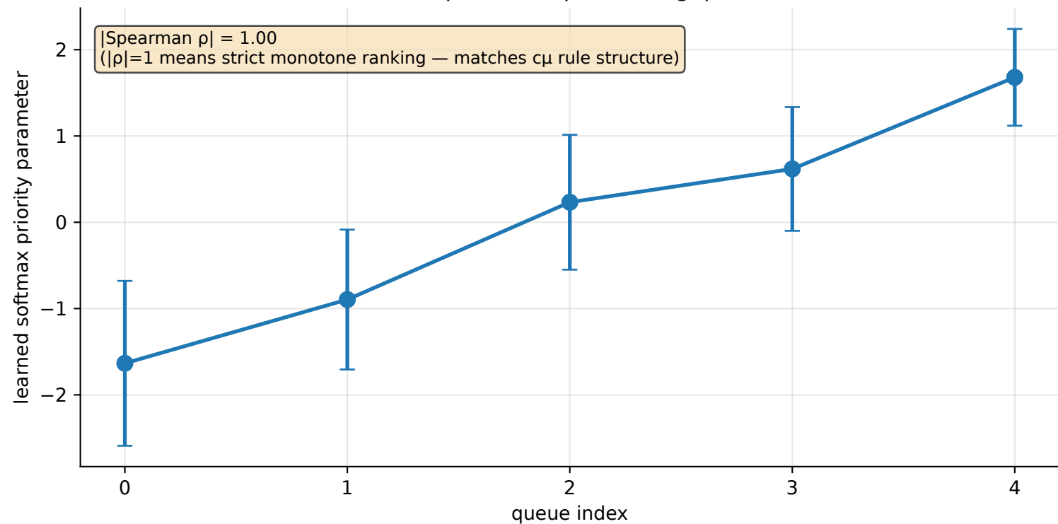
§5.2 Fig 9 left — learned policy ranks queues monotonically (cμ structure) (5-class, \rho=0.99 , \alpha=0.5 , \text{gap}=0.05 )
