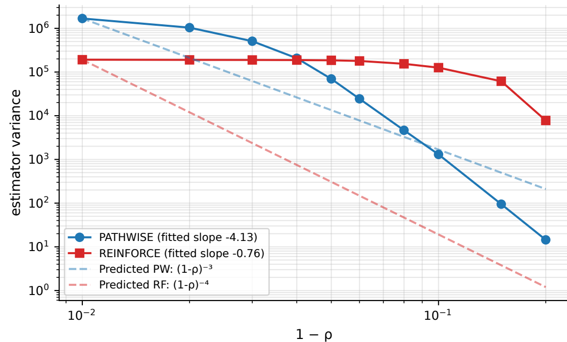
§8 Theorem 2 variance — fit deviates from predicted slope
