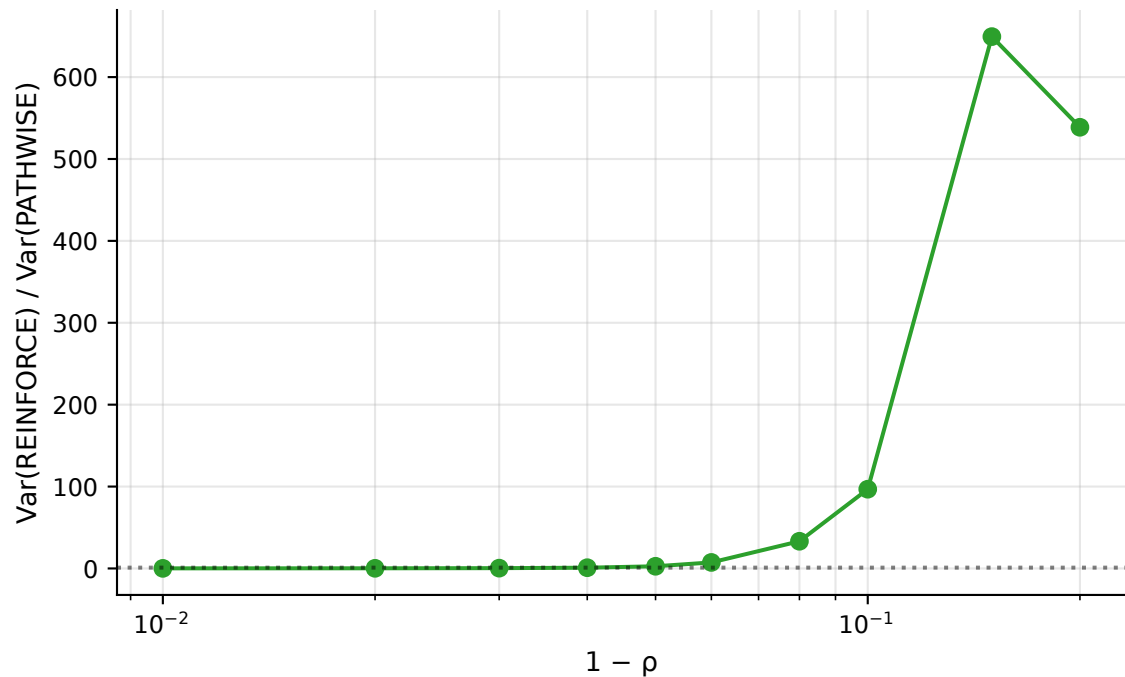
PATHWISE advantage vanishes as \rho \rightarrow 1 in our setup
