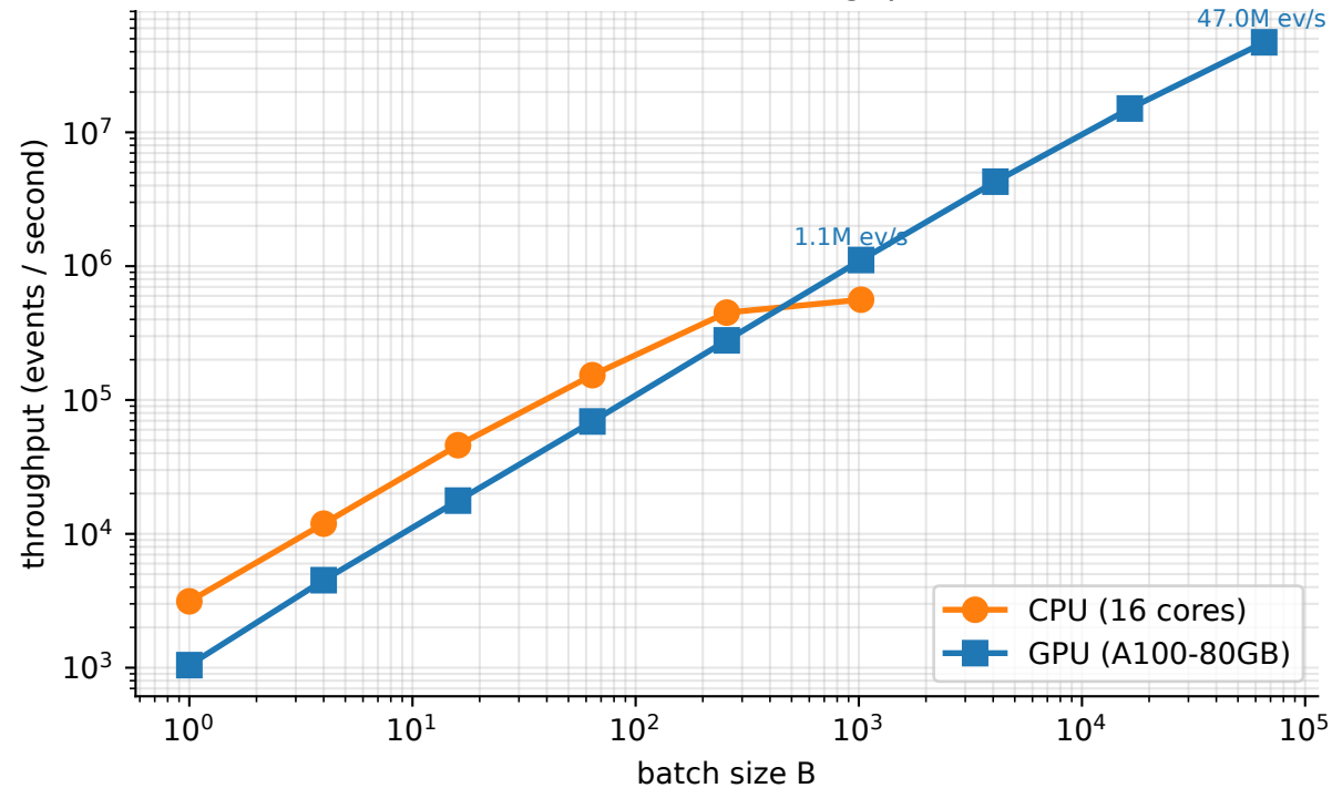
§4.3.1 PATHWISE simulation throughput — CPU vs GPU
