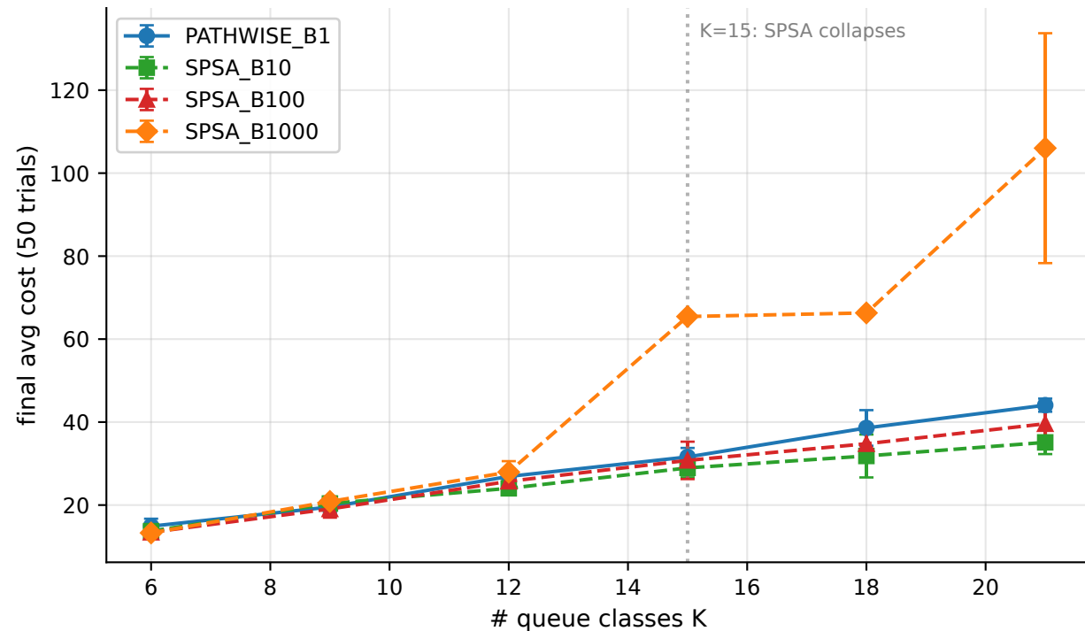
§5.3 Admission control — family reentrant_1
