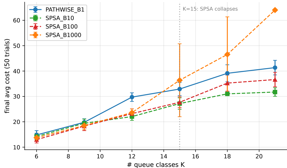
§5.3 Admission control — family reentrant_2
