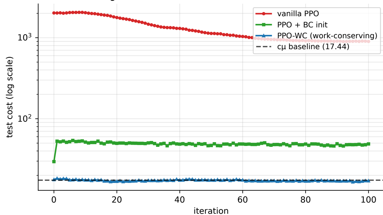
§6 Figure 12 (full) — PPO 3 variants on criss-cross
