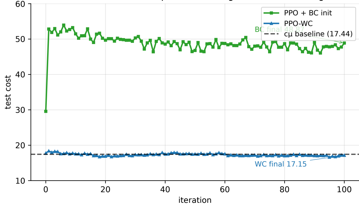
Zoom: PPO+WC < c\mu ; PPO+BC degrades over training
