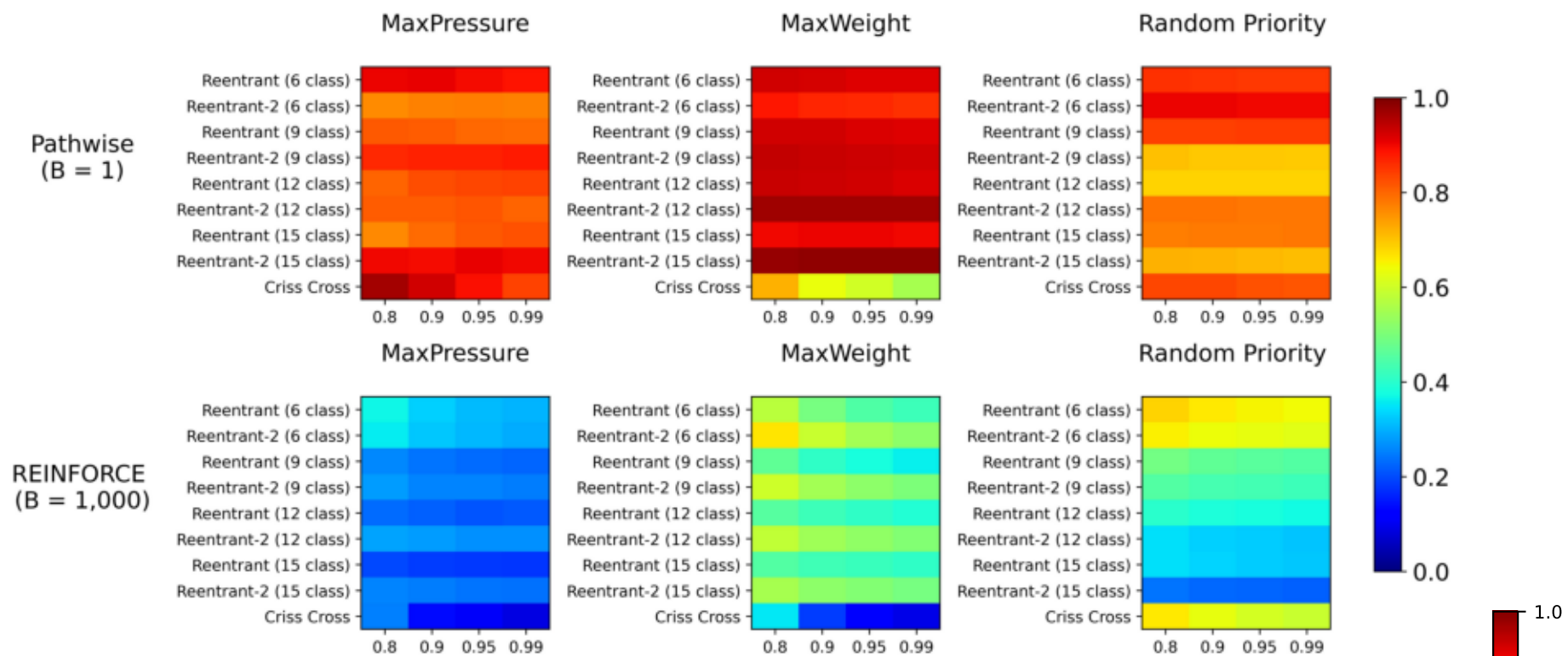
Paper Figure 8 (original; PATHWISE mostly \approx 1.0 )
