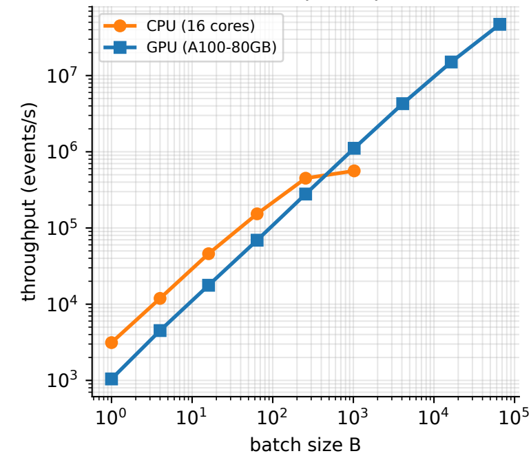
§4.3.1 GPU 84 \times speedup @ B=65K
