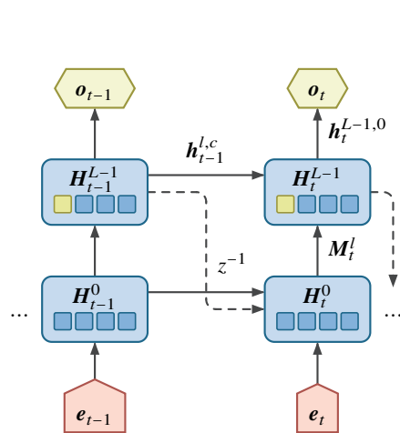
(a) grid over time and depth
