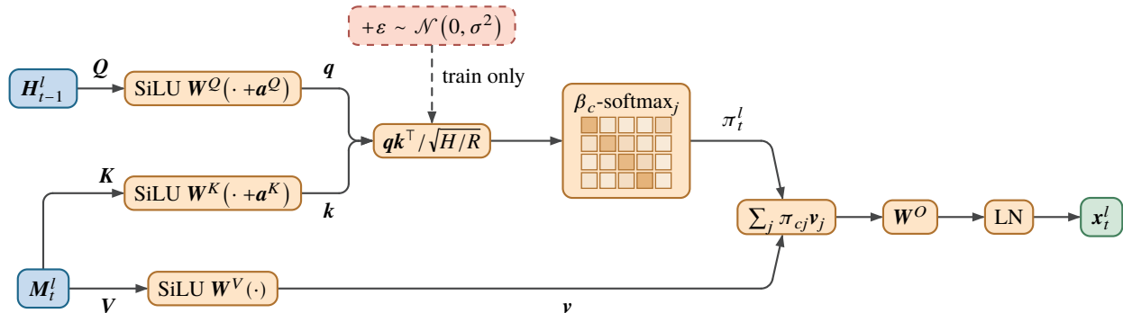
(c) inside the router of panel (b)
