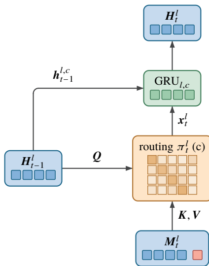
(b) one layer at timestep t
