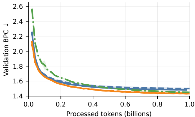
(a) text8 character modeling
