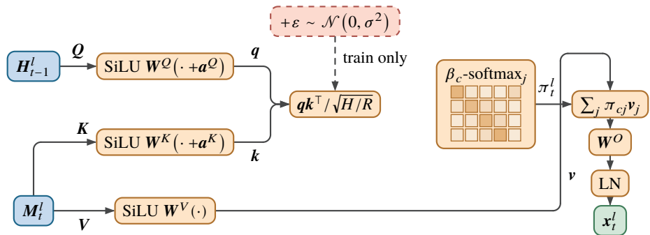
(c) inside the router of panel (b)
