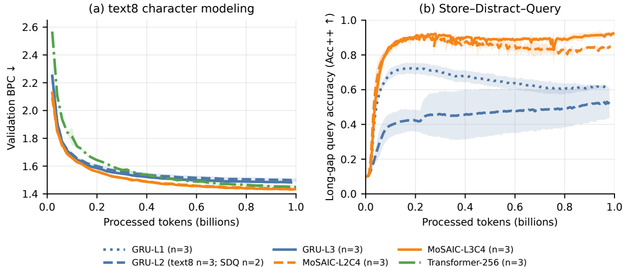
Figure 2: Learning dynamics under the standard 1B-token protocol. Lines show the mean across completed replicates and shading shows \pm 1 standard deviation. Text8 curves use three replicates; SDQ curves use three except GRU-L2, which uses two. (a) Validation BPC on text8. (b) Online long-gap query accuracy on SDQ. Final SDQ values in Table 1 use the mean of each replicate’s last five logged values.
