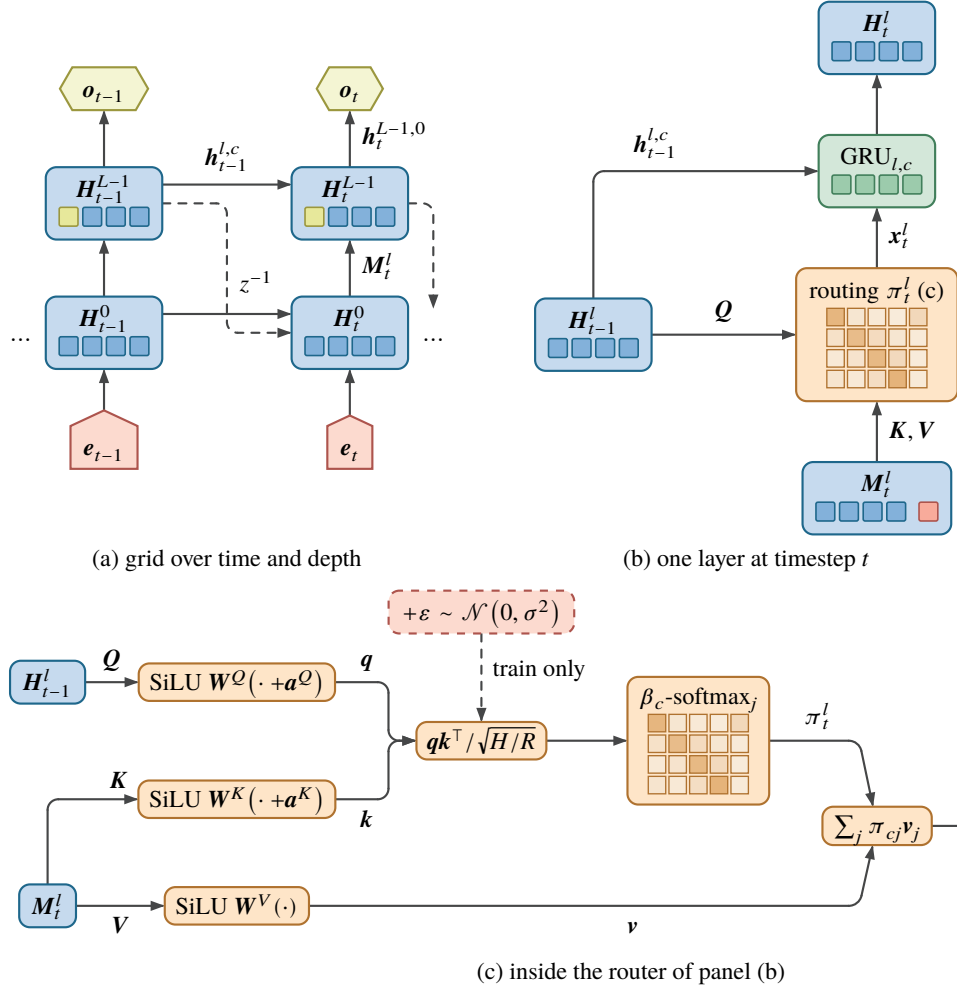
Figure 1: MoSAIC mechanism. At timestep t , each persistent column state queries a layer-specific message bank. The first layer reads the current input together with the previous top-layer column states; later layers read the newly updated states below them. The routed message is the input to an independent recurrent update. All top-layer column states are carried to timestep t + 1 .
