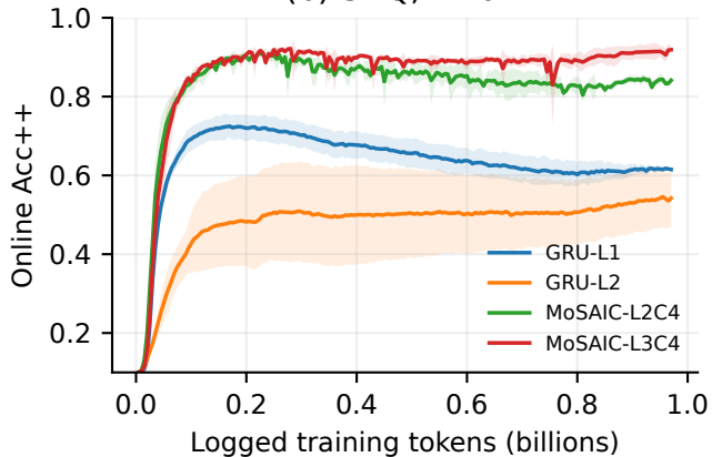
(b) SDQ, ~10M
