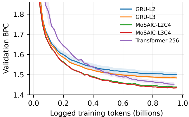
(a) Text8, ~10M
