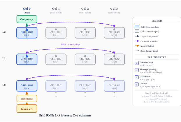
Figure 1: Grid RNN architecture. Cells are arranged in an L \times C grid. At each timestep, each column independently processes its input (column 0 receives the embedded token; others receive zero), then all columns exchange information via multi-head attention with learnable column identity keys. Different columns converge to distinct memory roles without explicit supervision.
