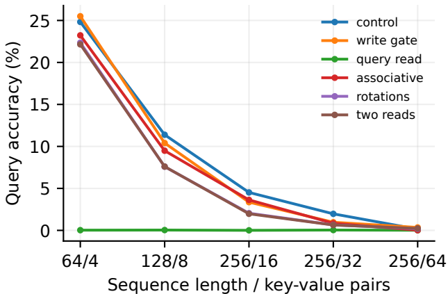
(b) MQAR, seed 42
