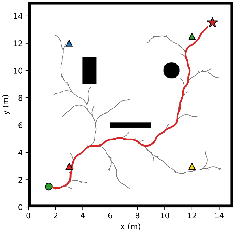
open: Dubins RRT, 356 iterations
