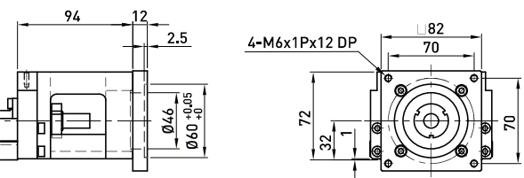
Motor connection flange F4
