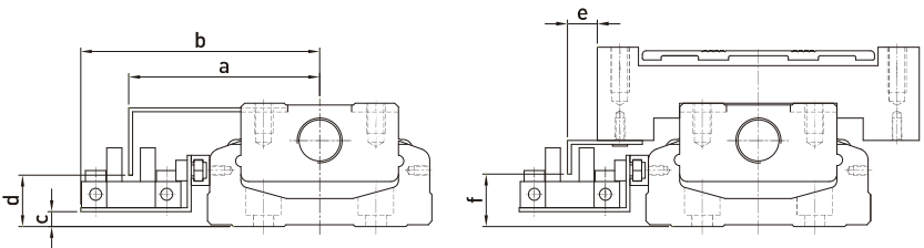
Limit switch S1: PM-L45
