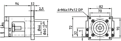
Motor connection flange F4
