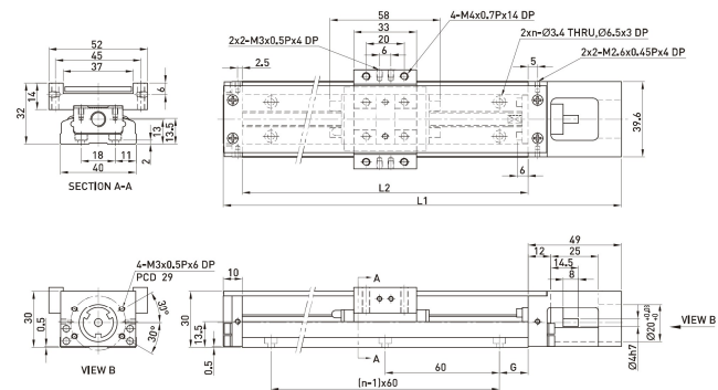
DK40 Including protective cover
