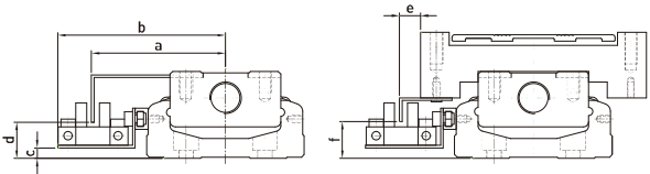
Limit switch S1: PM-L45
