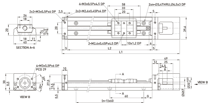
DK40 Excluding protective cover
