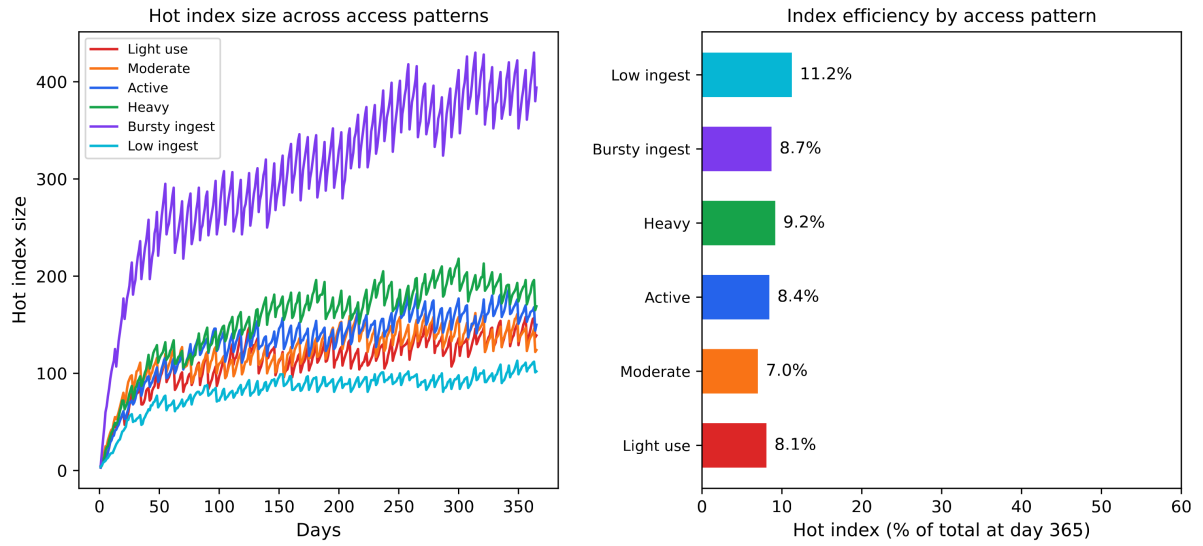
Figure 3: Tiered storage scaling across six access patterns over one simulated year. Left: Hot index size over time. All scenarios plateau; absolute size scales with ingestion rate but growth converges to zero. The bursty ingest scenario (10 memories/day, 2 queries/day) shows the most variance but still stabilises. Right: Hot index as percentage of total memories at day 365. All scenarios converge to the 7–11% range, indicating that bounded hot index size is robust to access pattern variation.
