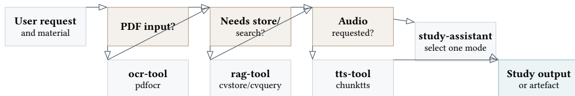
Figure 6: Agent decision flow across study modes and tool handoffs.
