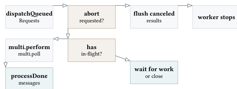
Figure 12: Worker control flow in the relay HTTP transport library.
