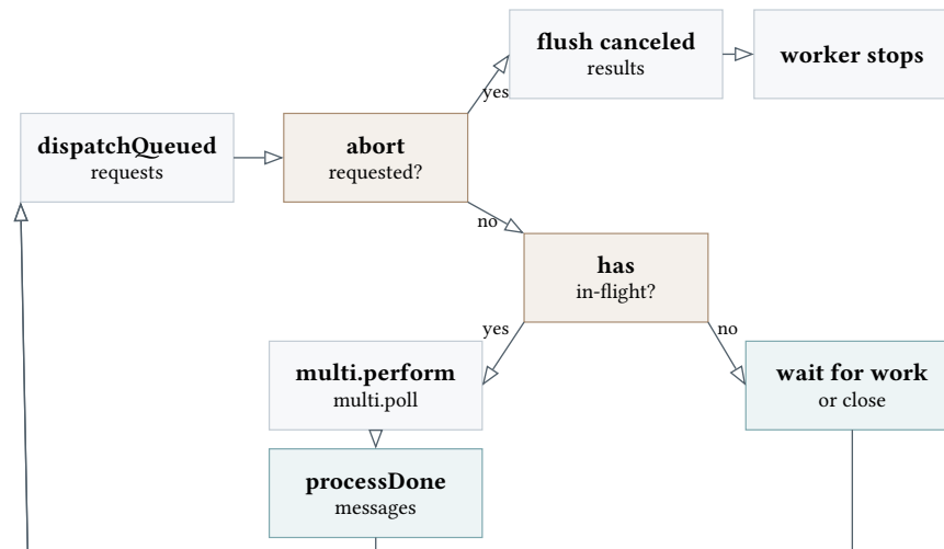
Figure 12: Worker control flow in the relay HTTP transport library.
