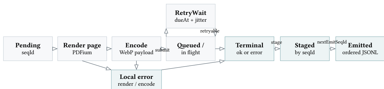
Figure 7: Per-page state machine in the pdfocr OCR pipeline.
