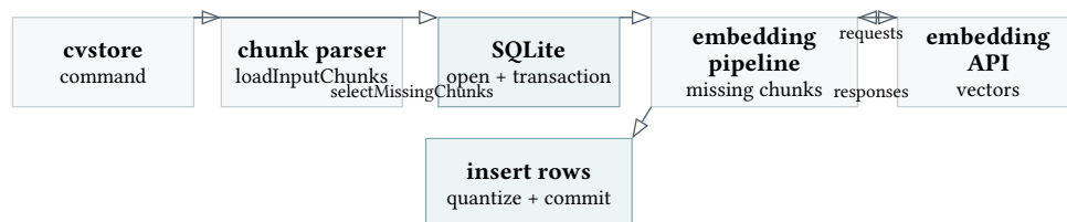
Figure 10: chunkvec ingest sequence from marked chunks to committed vectors.
