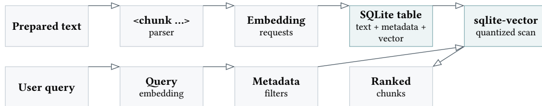
Figure 3: RAG storage and retrieval data flow.
