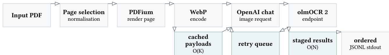
Figure 2: OCR data flow from PDF pages to ordered JSONL records.
