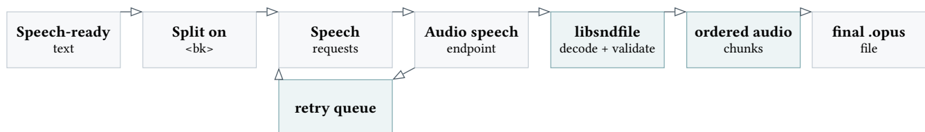
Figure 4: TTS data flow from speech-prepared text to final .opus artefact.
