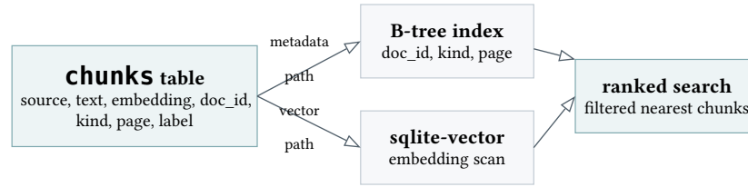
Figure 9: chunkvec storage schema and retrieval indexes.
