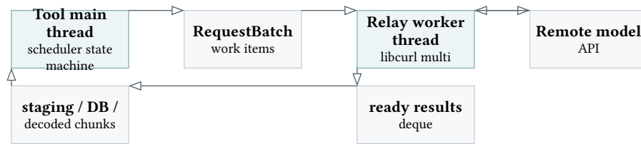
Figure 5: Component interaction between a core tool and the relay transport layer.
