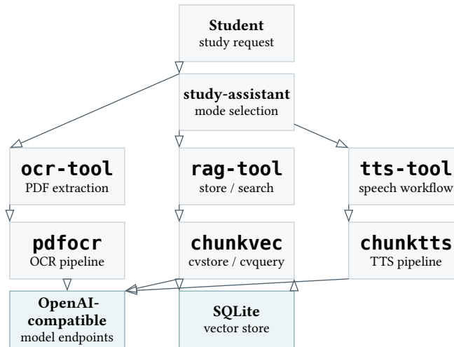
Figure 1: Global architecture of the study-assistant system.
