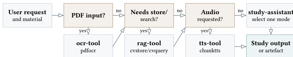
Figure 6: Agent decision flow across study modes and tool handoffs.
