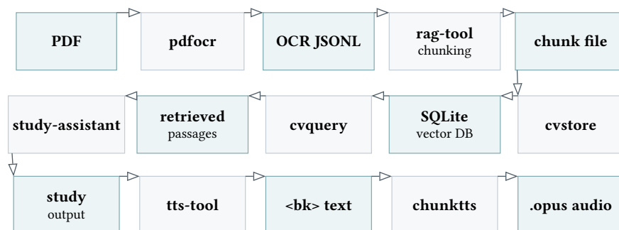
Figure 13: Concrete artefact chain across OCR, retrieval, study generation, and TTS.
