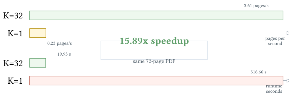
Figure 13: OCR throughput benchmark showing runtime reduction and throughput increase under bounded concurrency.
