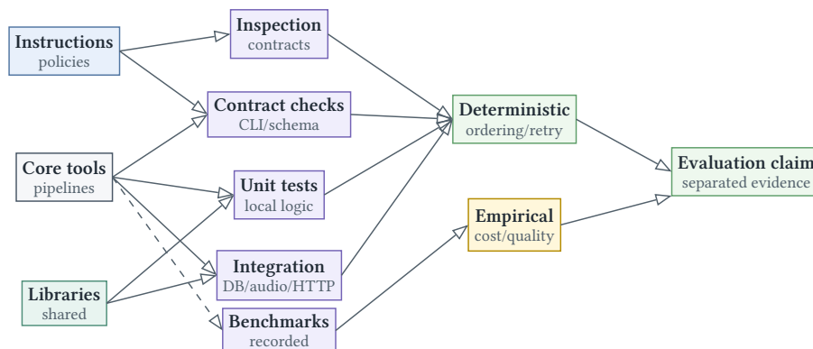
Figure 12: Verification evidence topology separating deterministic implementation evidence from empirical model and performance evidence.
