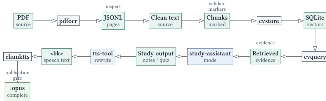
Figure 11: Artefact lineage across OCR, retrieval, study generation, and optional audio publication.
