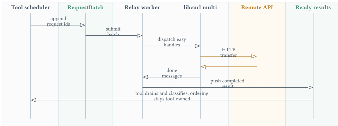
Figure 10: Relay concurrency boundary between tool-owned scheduler state and worker-owned libcurl multiplexing.
