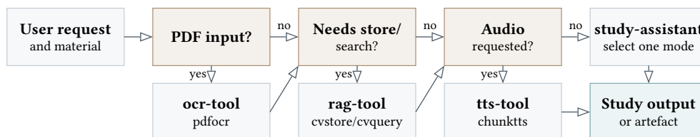
Figure 6: Agent decision flow across study modes and tool handoffs.
