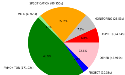
junit (19.061s)
