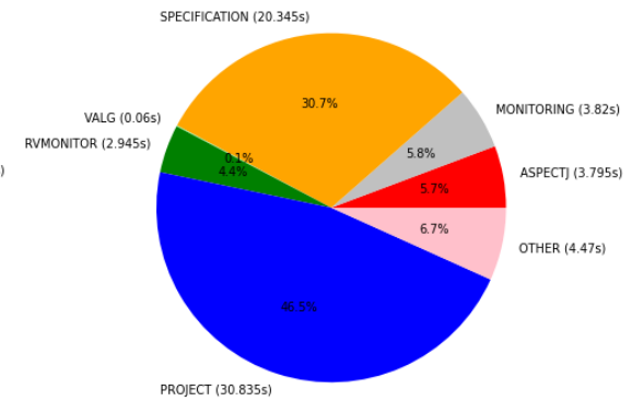
geogrid (25.269s)
