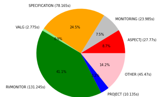
junit (19.061s)
