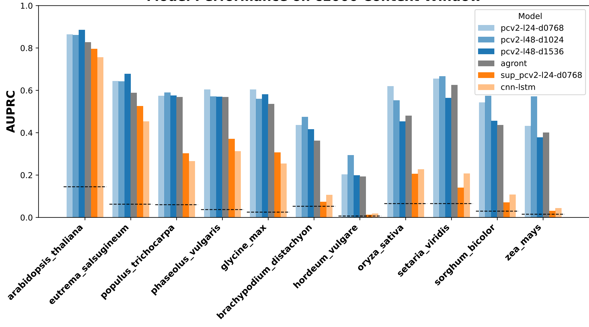
Model Performance on c1000 Context Window
