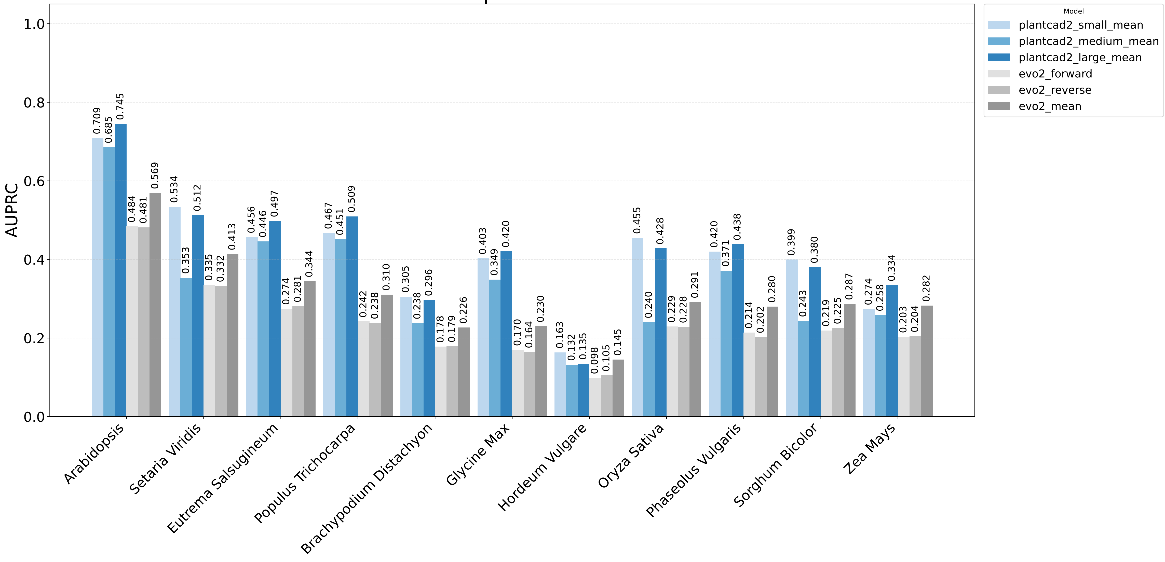
Model Comparison: XGBoost
