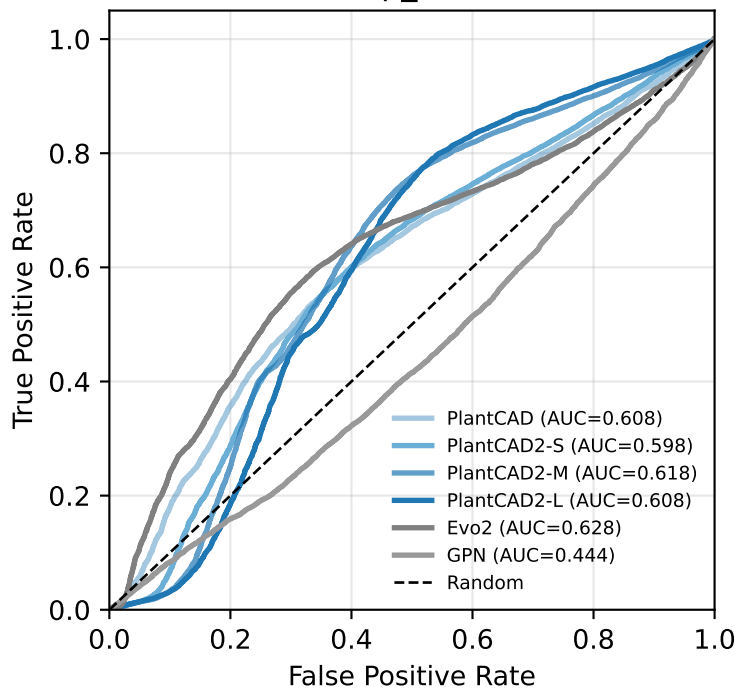
stop_sites
