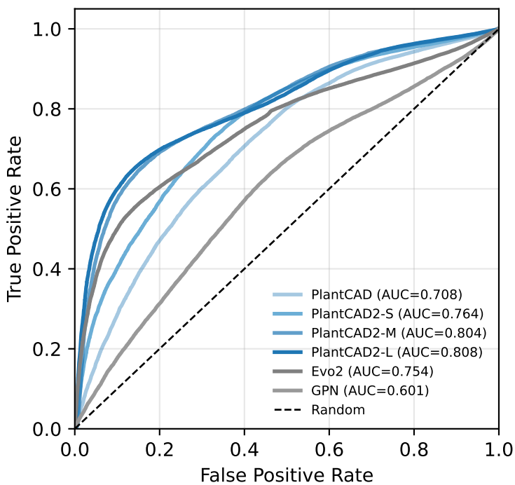
donor
