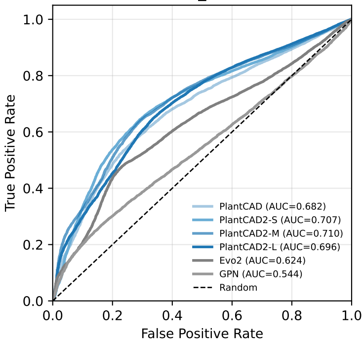
start_sites
