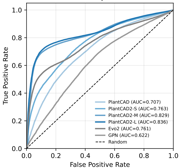
acceptor
