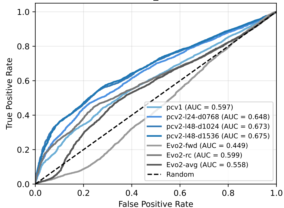
donor
