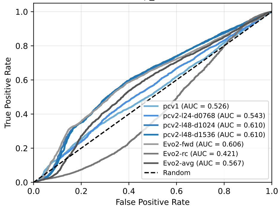
acceptor
