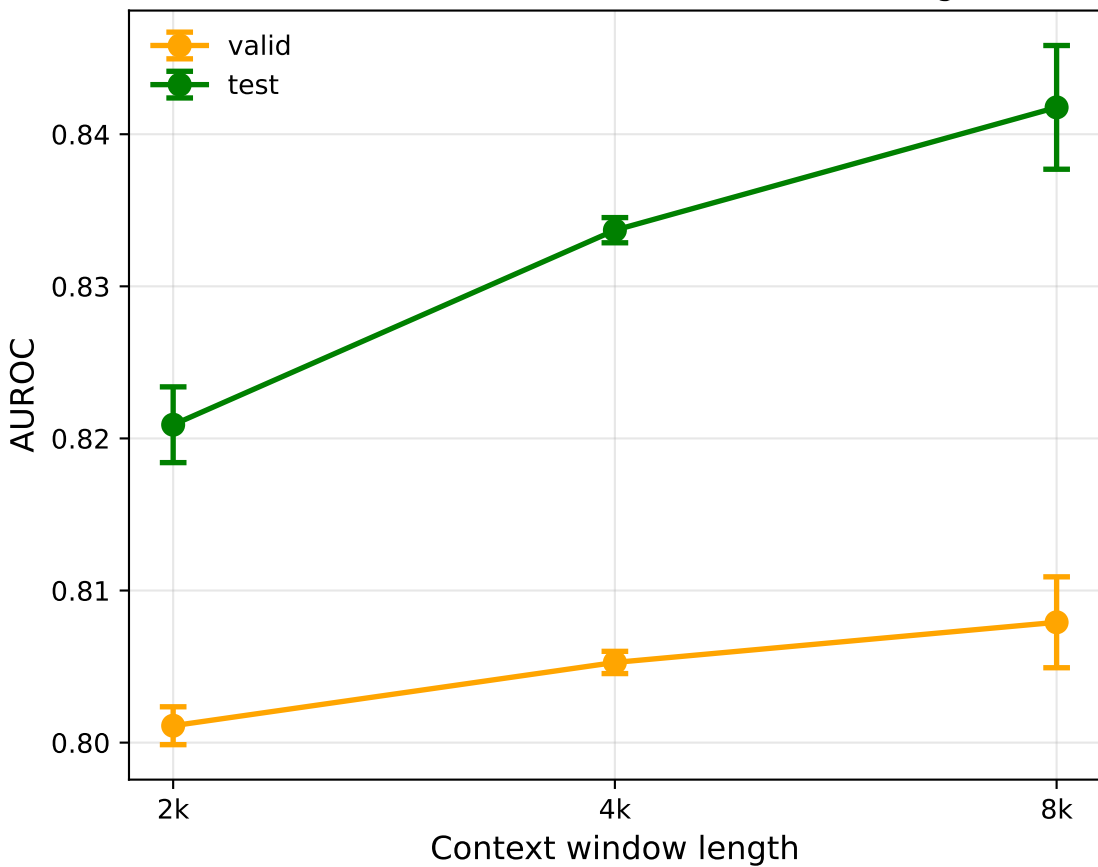
Model Performance vs Context Window Length
