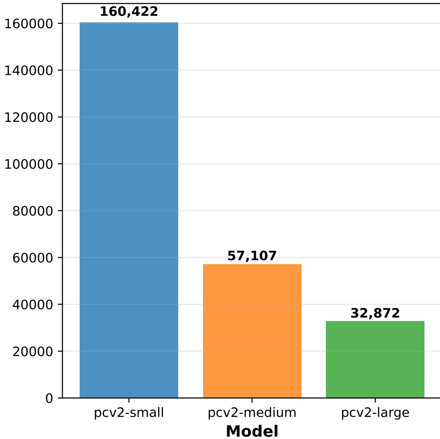
Total Throughput (tokens/sec)
