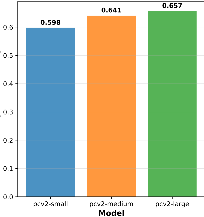
MLM accuracy (15% masking rate)
