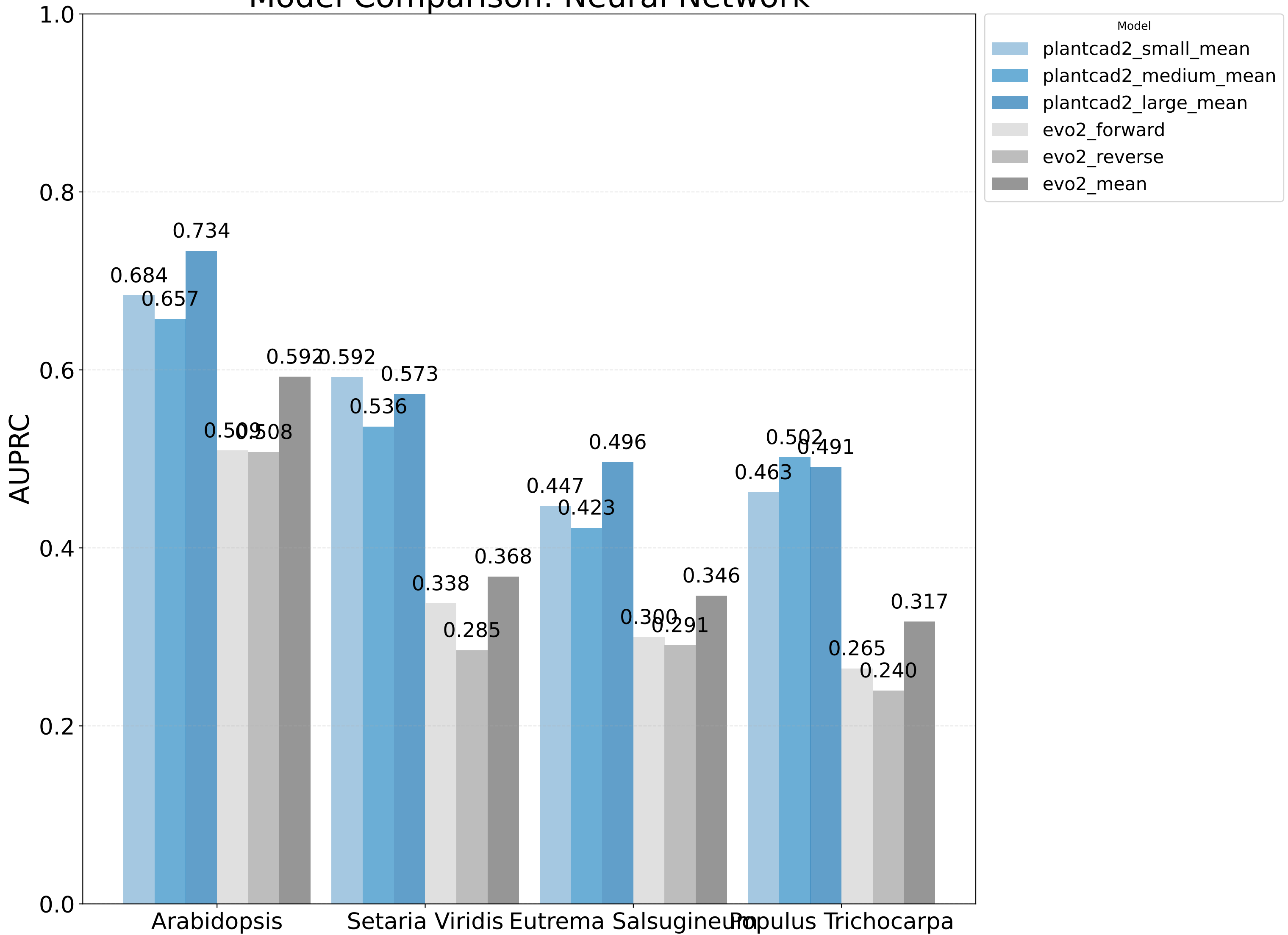
Model Comparison: Neural Network
