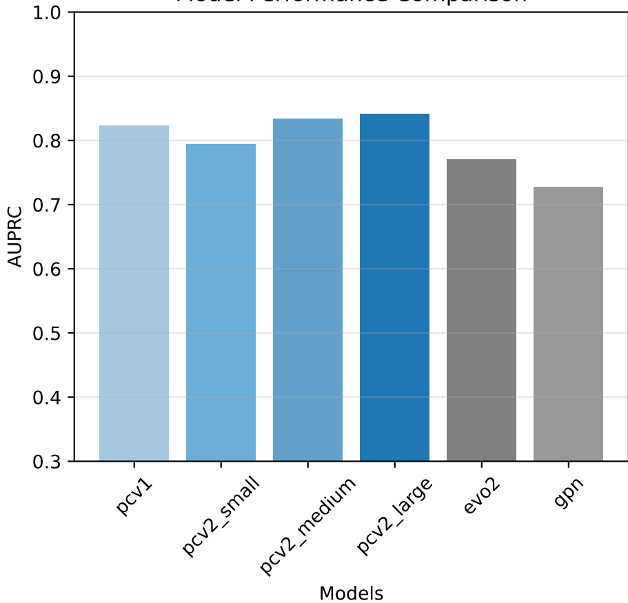
Model Performance Comparison
