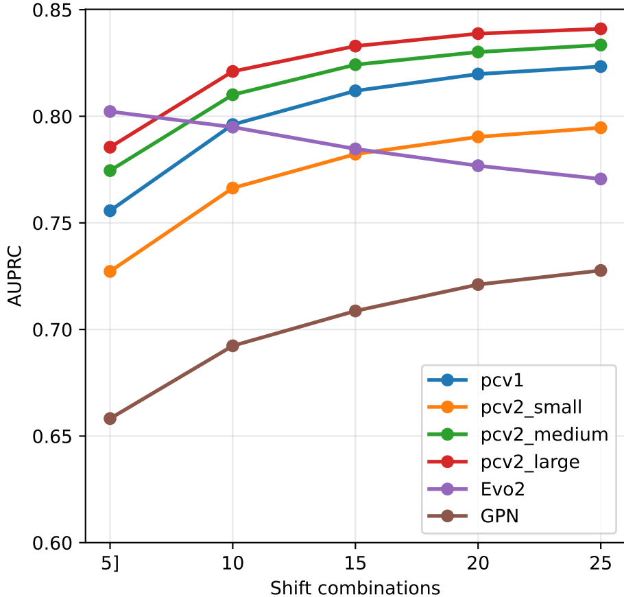
AUPRC Performance Across Cumulative Shift Combinations
