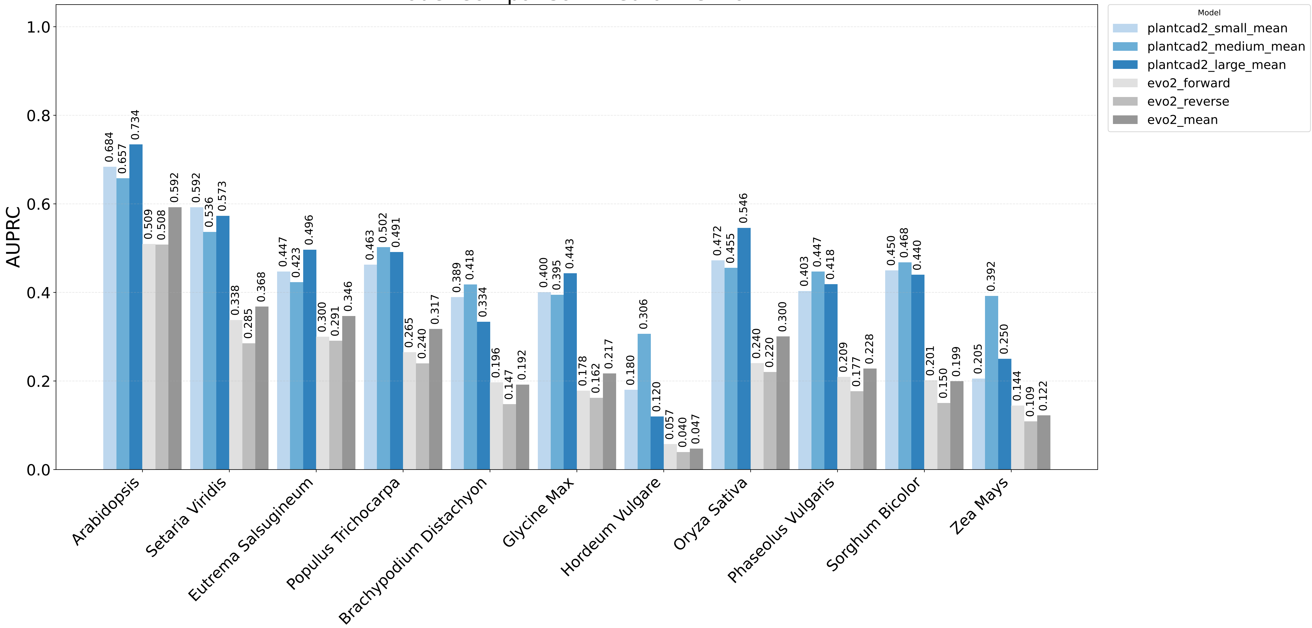
Model Comparison: Neural Network
