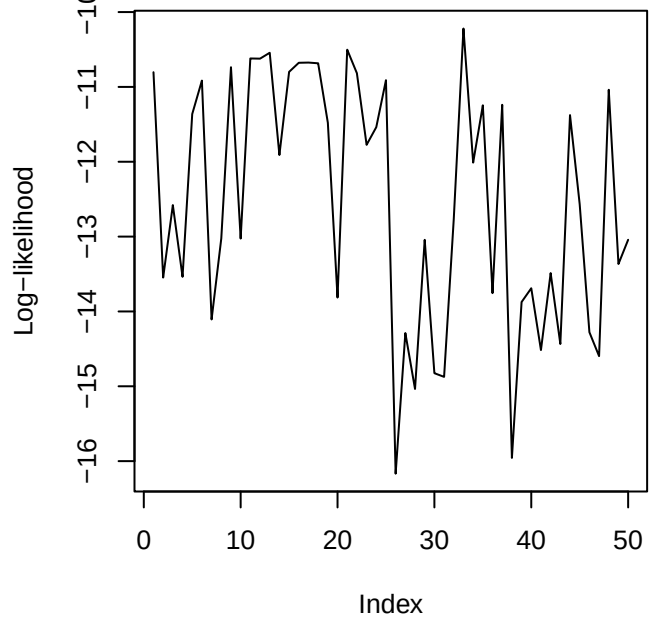
Traceplot of the log-likelihood
