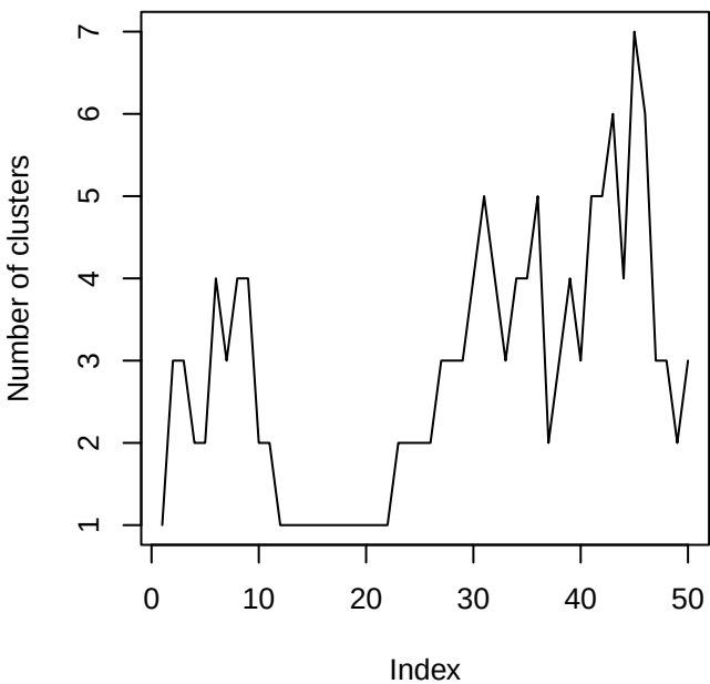
Traceplot of the number of clusters
