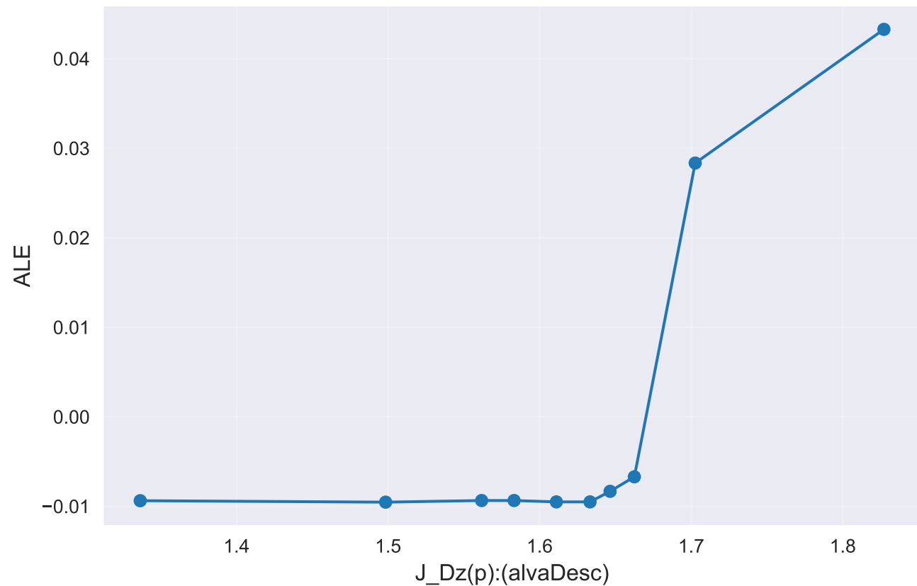
ALE plot: J_Dz(p):(alvaDesc) CatBoost__model_specific_best_subset__rank_top_20
