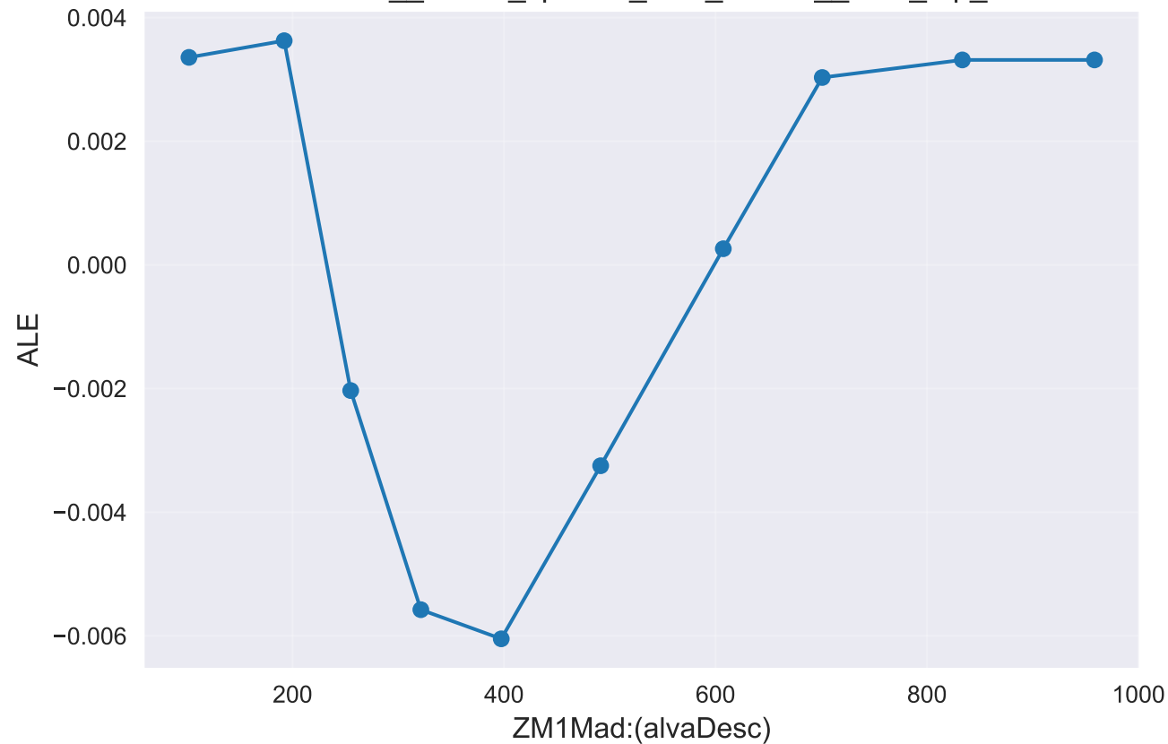
ALE plot: ZM1Mad:(alvaDesc) CatBoost__model_specific_best_subset__rank_top_20
