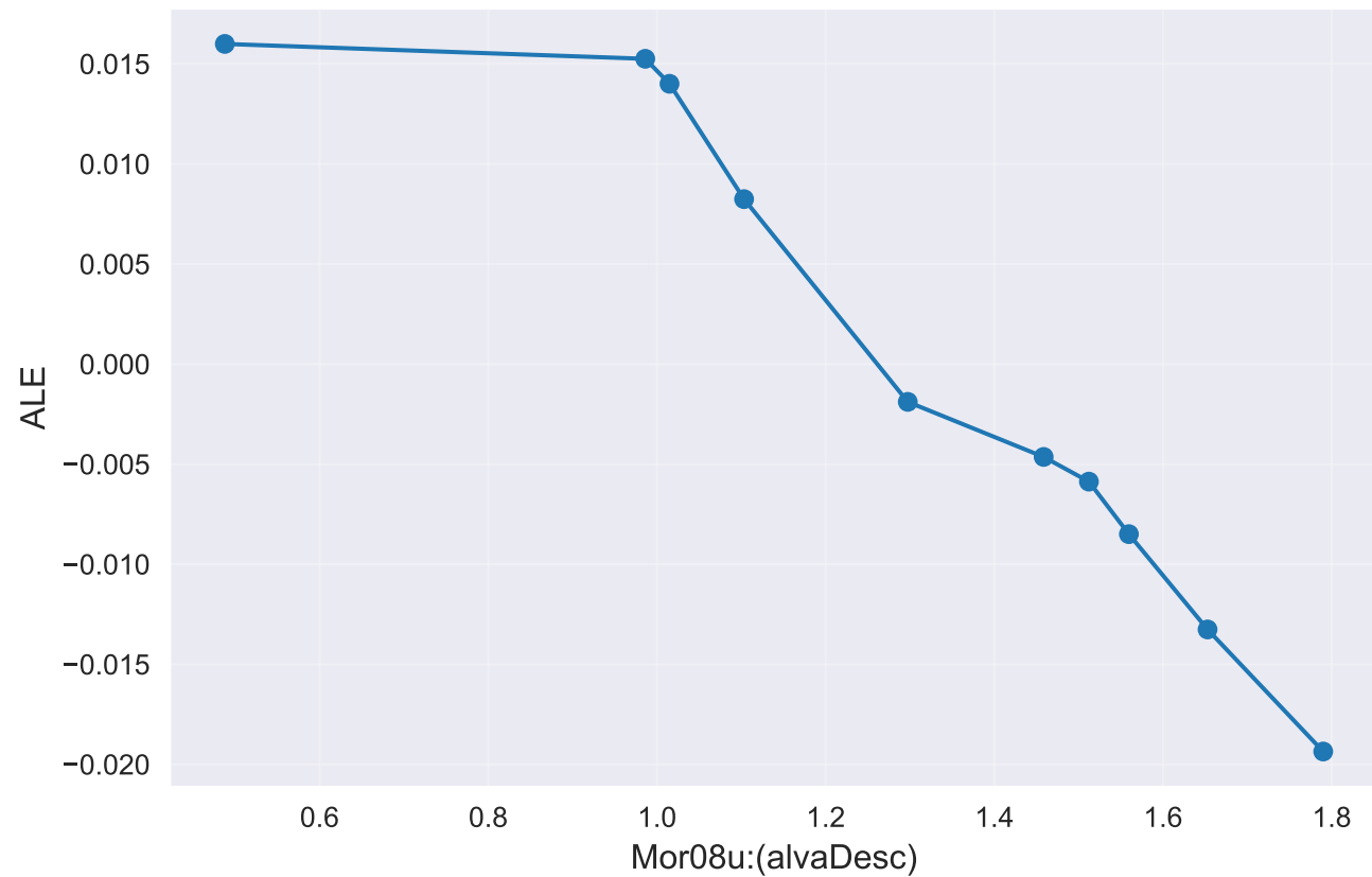
ALE plot: Mor08u:(alvaDesc) GaussianProcess__model_specific_best_subset__rank_top_20
