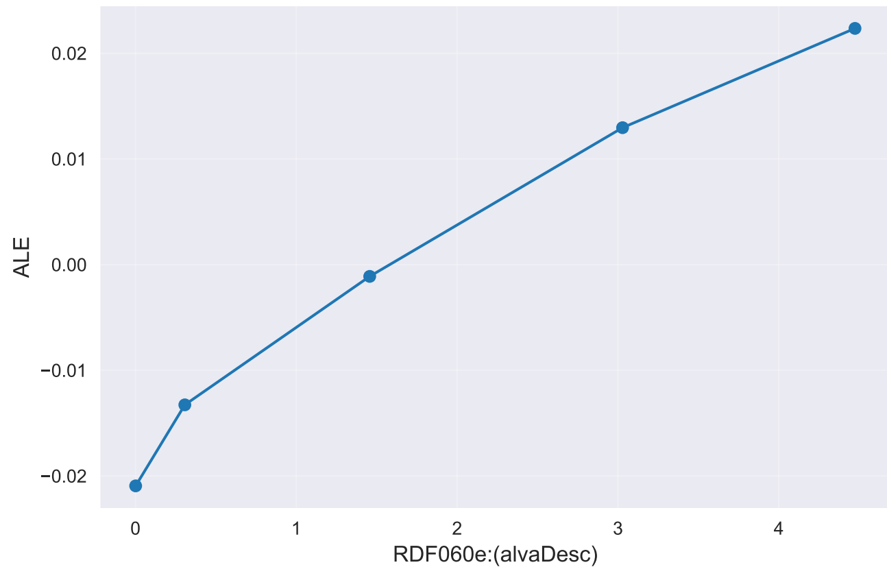
ALE plot: RDF060e:(alvaDesc) GaussianProcess__model_specific_best_subset__rank_top_20
