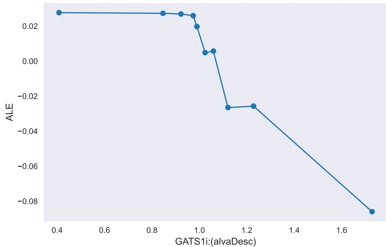
ALE plot: GATS1i:(alvaDesc) GradientBoosting__model_specific_best_subset__rank_top_20
