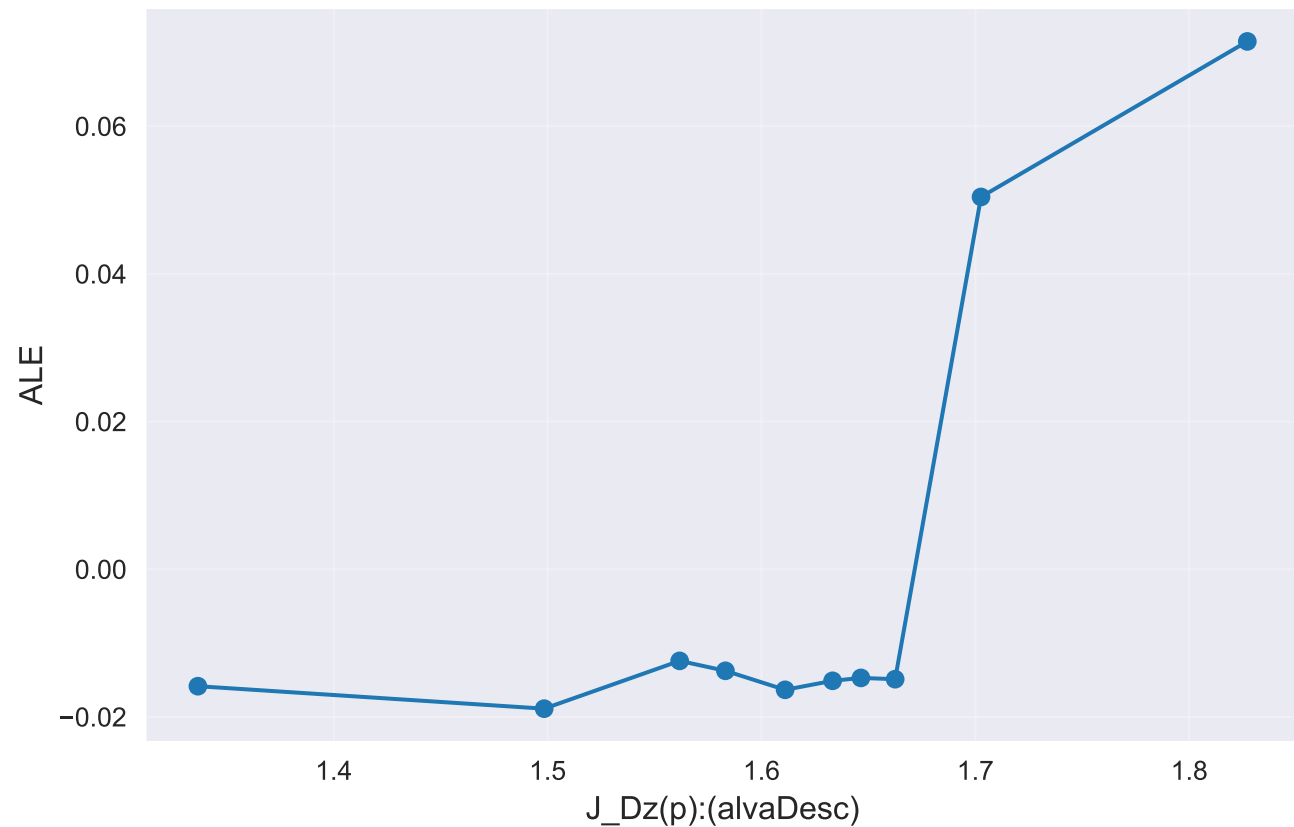
ALE plot: J_{Dz(p)}:(\text{alvaDesc}) GradientBoosting__model_specific_best_subset__rank_top_20
